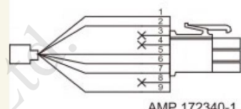
AMP 172340-1
